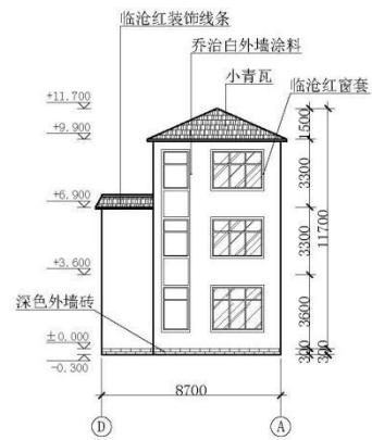
④—① 轴立面图1:200
